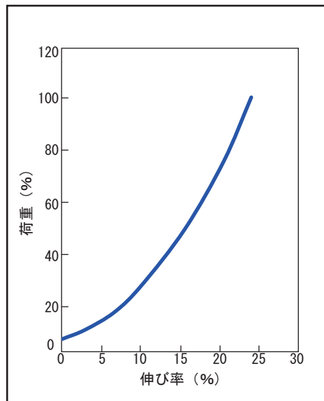
荷重・伸び率曲線(50mm)
